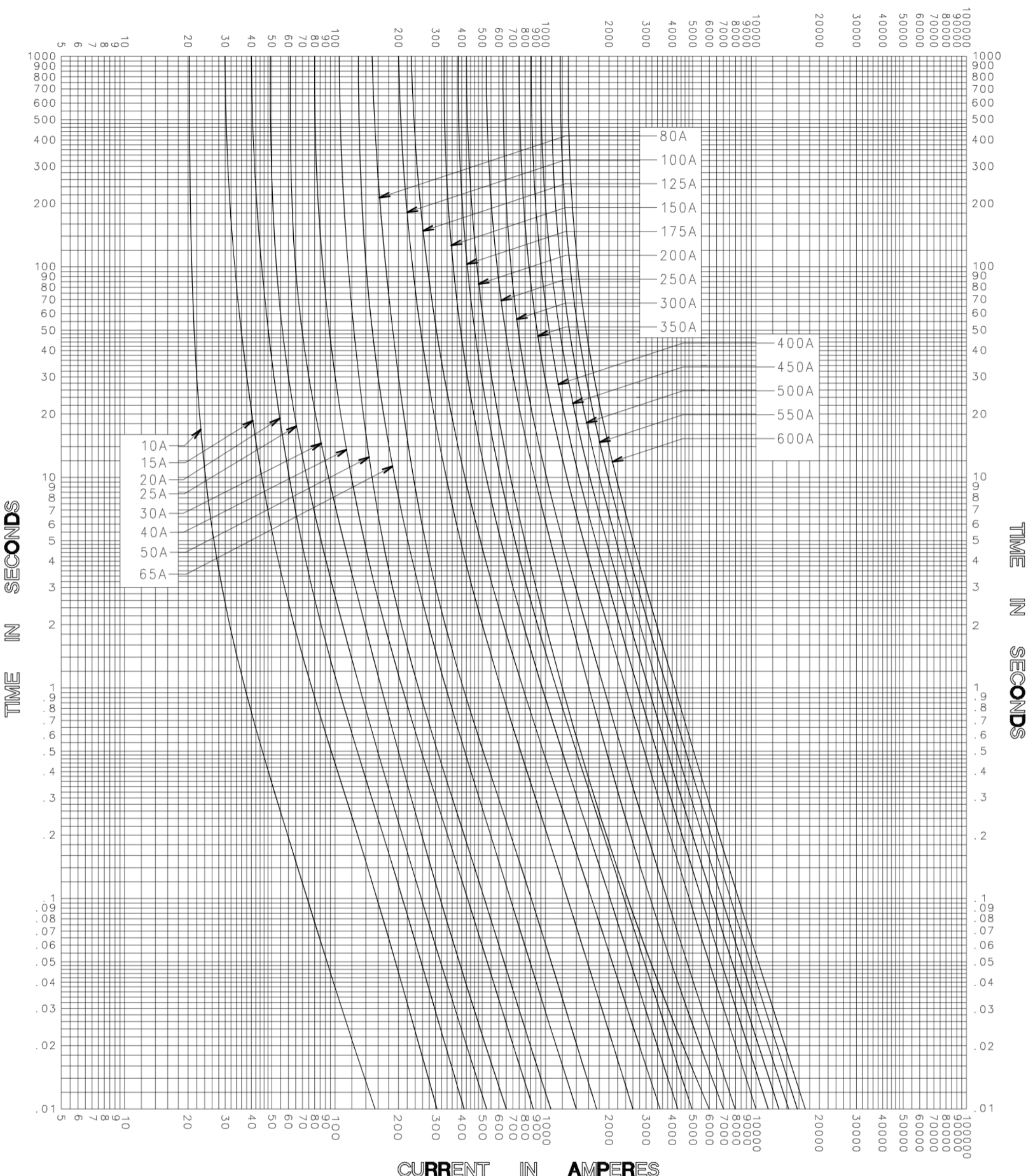
MELTING TIME CURRENT CHARACTERISTIC CURVES
