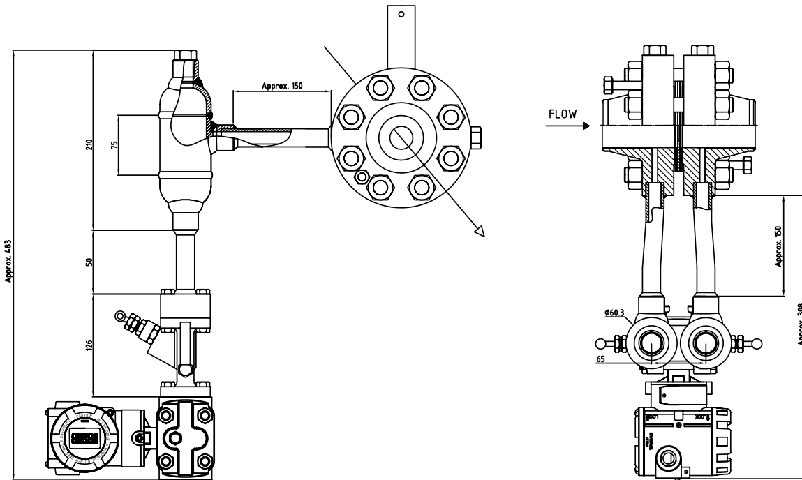
Side View
