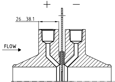
Corner tap
