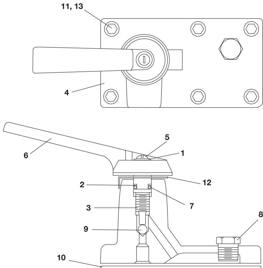
Figure 1, VM-2 Manual Valve
