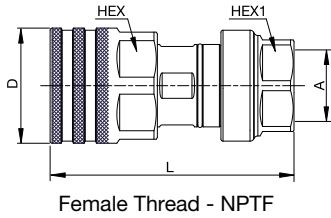
Female Thread - NPTF
