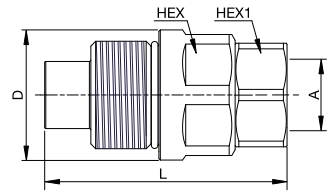
Female Thread - NPTF
