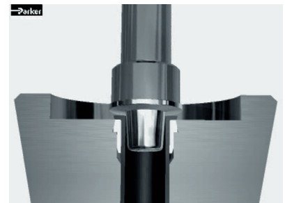
The front surface is continuously rolled and compressed. From the inside, the tube surface is slightly expanded to clamp the sleeve
