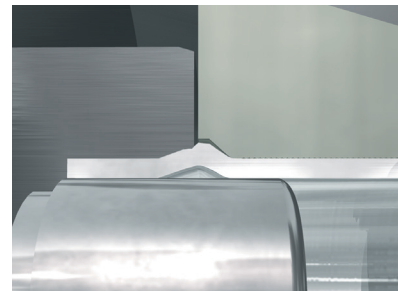
The inner contour also gets slightly deformed but remains smooth and unrestricted for good flow characteristics
