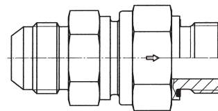
Triple-Lok® 37° flare end / Male metric thread – ED-seal (ISO 9974)
