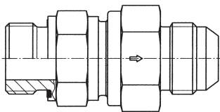
Male metric thread – ED-seal (ISO 9974) / Triple-Lok® 37° flare end
