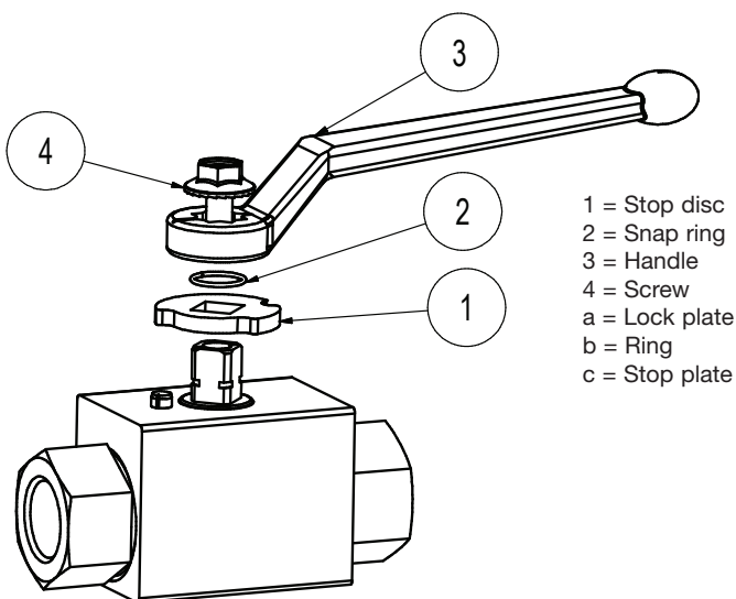
Disassembly
