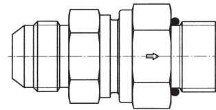
Triple-Lok® 37° flare end / Male UN/UNF thread – O-ring (ISO 11926)
