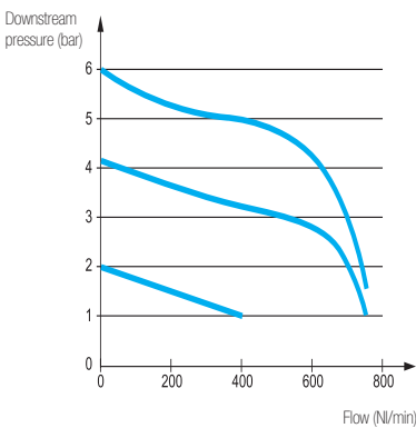
G1/8 Models
