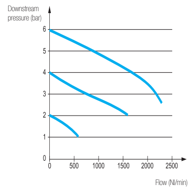
G3/8 Models
