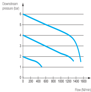
G1/4 Models
