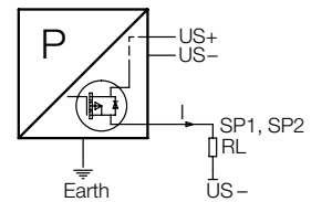
Connection of loads to switching output
